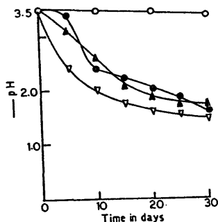
Fig. 2 Decrease in pH in media by a) iron & sulphur oxidising bacteria ▽ b) sulphur oxidising bacteria ● Δ
