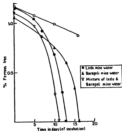
Fig.1 Decrease in Ferrous Iron conc. in media by growing culture of a) Iron & sulphur oxidising bacteria \nabla b) Iron oxidising bacteria \bullet \Delta
